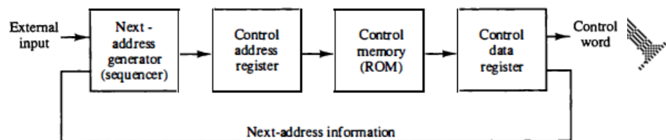
Figure 7-1 Microprogrammed control organization.
