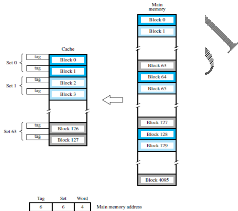
Figure 8.18 Set-associative-mapped cache with two blocks per set.
