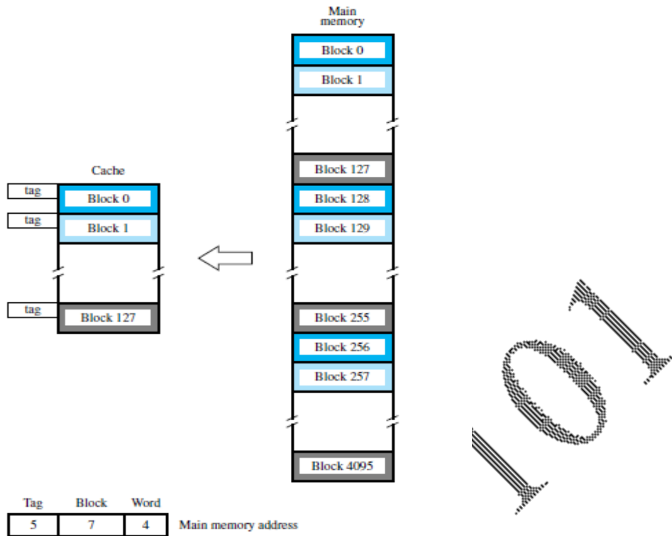
Figure 8.16 Direct-mapped cache.
