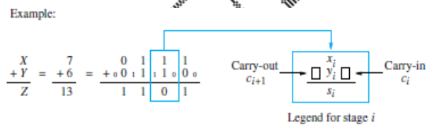
Figure 9.1 Logic specification for a stage of binary addition.
